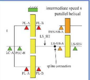
Gearbox vulnerability map TRL3
