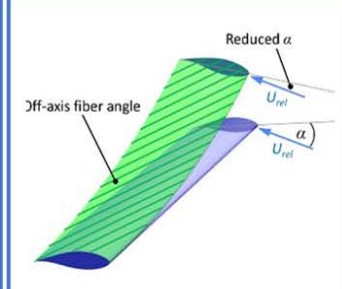
Buckling resistant blades TRL3
