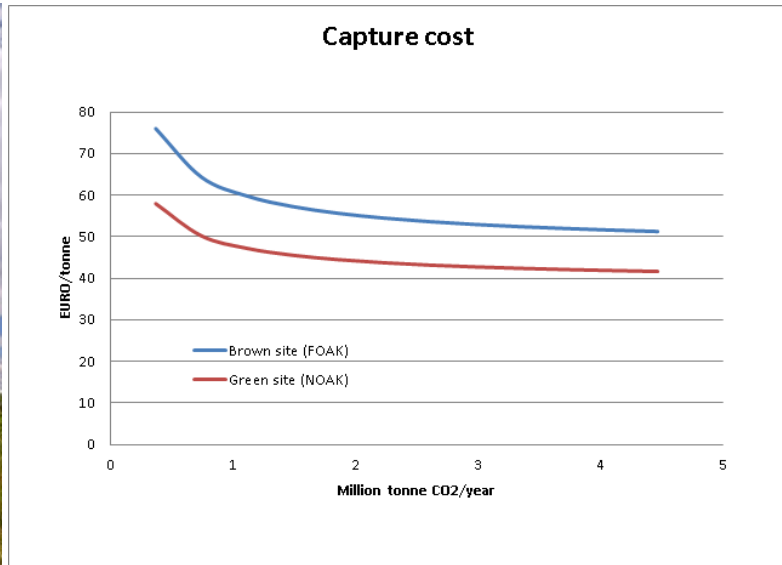
Figure 8: Economy of Scale for Natural Gas Sweetening Capture Costs
